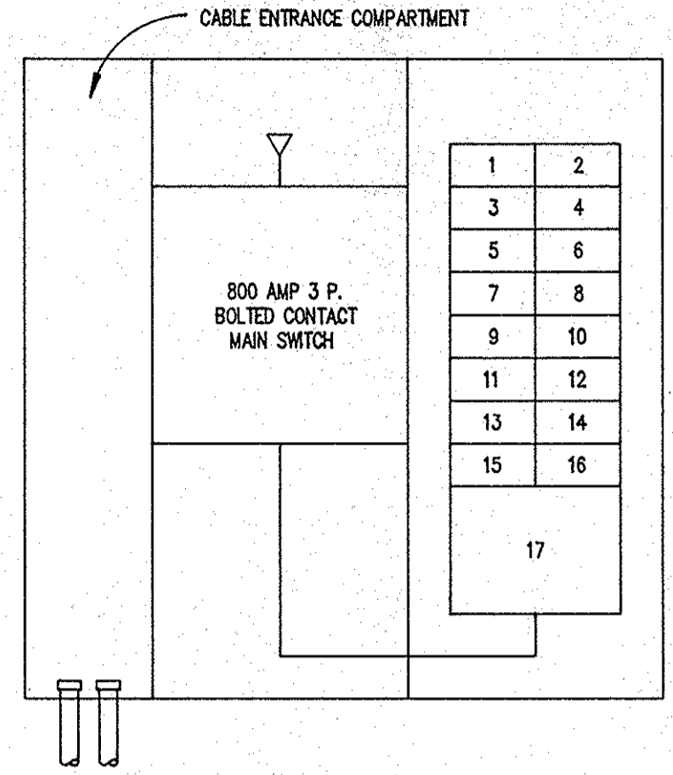
SWITCHBOARD "M" 120/208V 3Ø 4W WYE 800 AMP BUS
