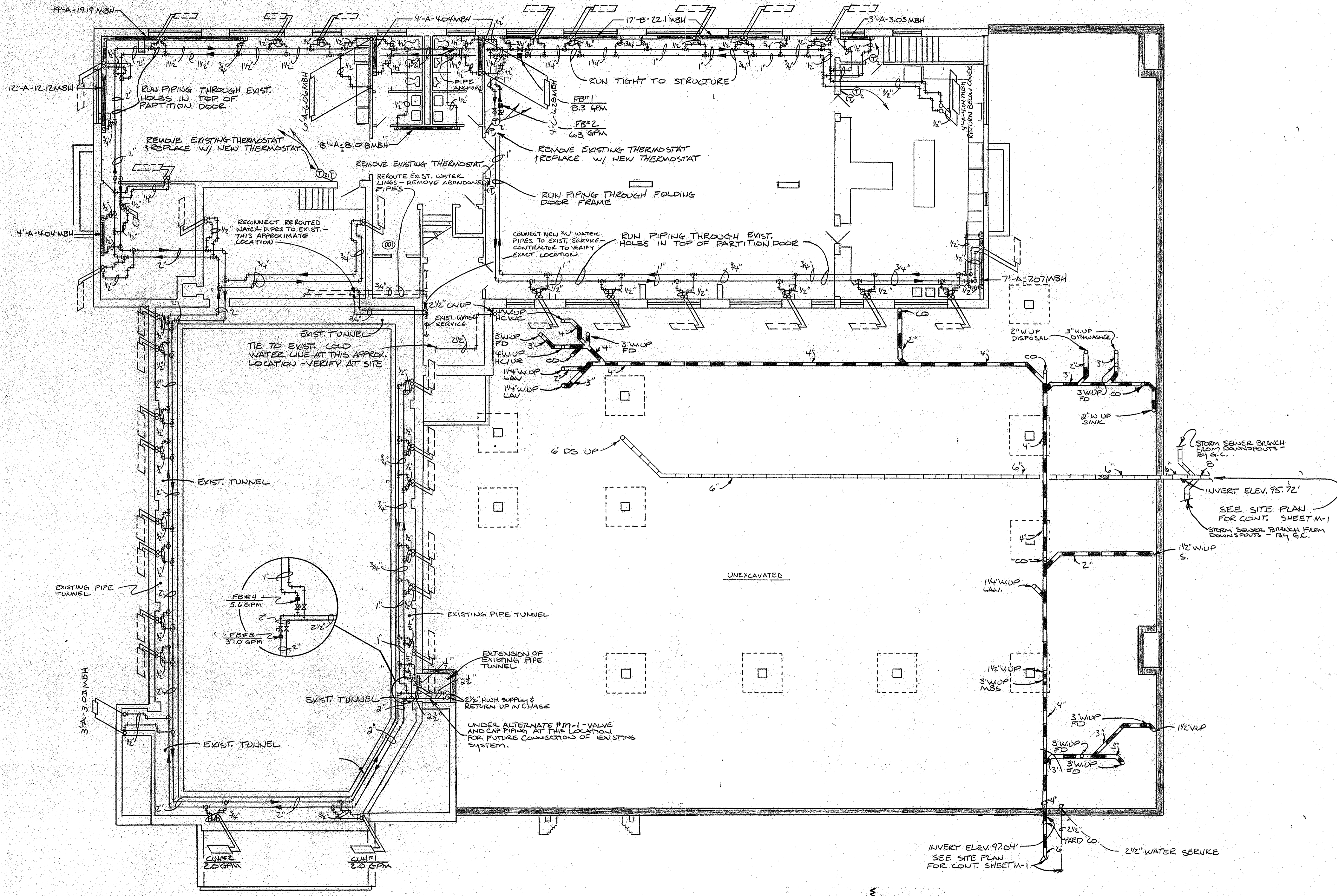
BASEMENT FLOOR PLAN - PLUMBING & HEATING SCALE: 1/8" = 1'-0"
